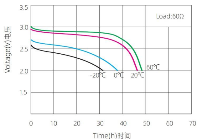
Temperature Characteristics 温度特性
