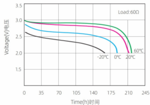
Temperature Characteristics 温度特性
