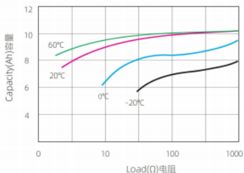
Capacity vs Resistance 容量vs电阻
